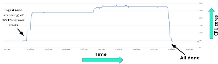
Figure 3. Example of cluster scaling on the Arkivum solution.
